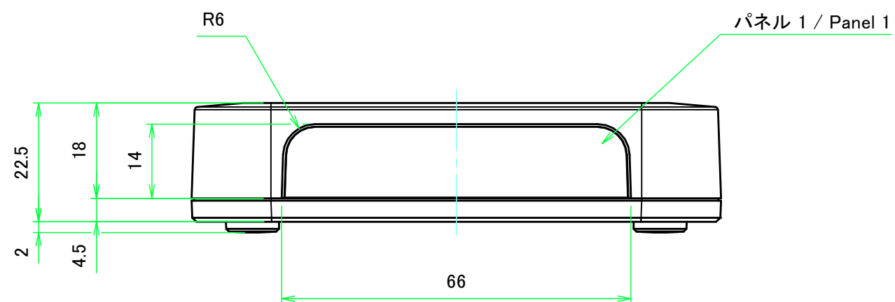
B-B (1:1)
